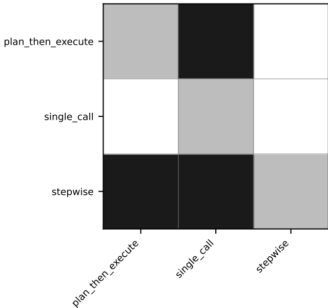
paradigm - total_tokens
