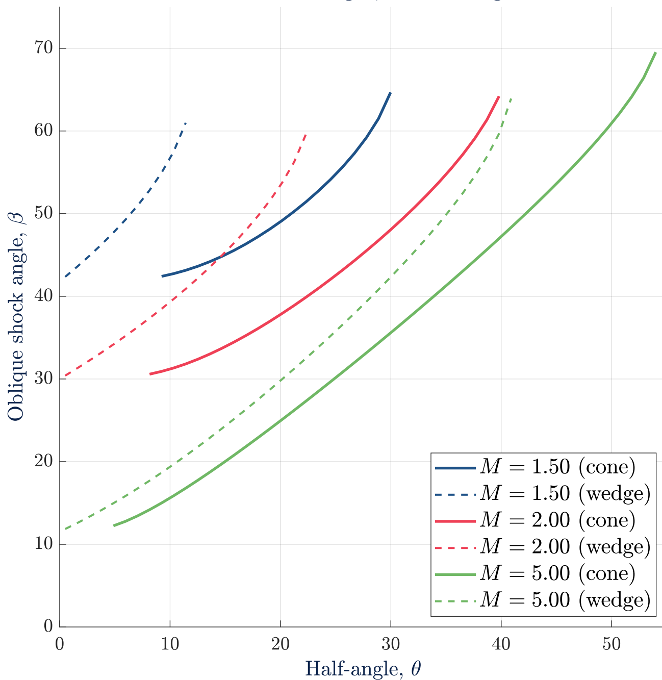
Conical Shock angle \beta_c vs half-angle \theta_c
