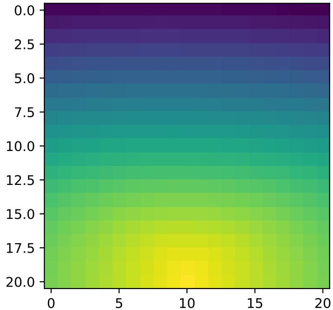
Energy (True)
