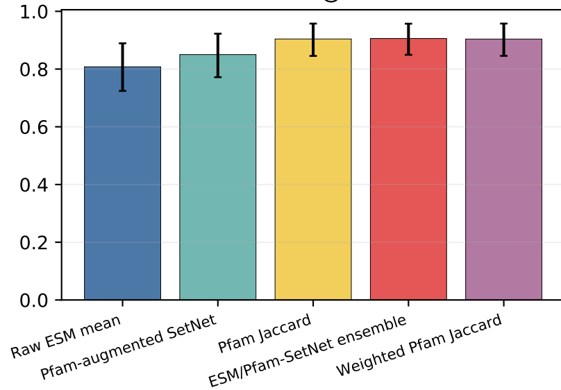
nDCG@50
