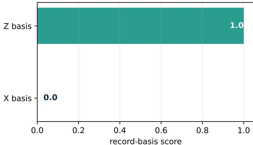
Two-record GHZ diagnostic
