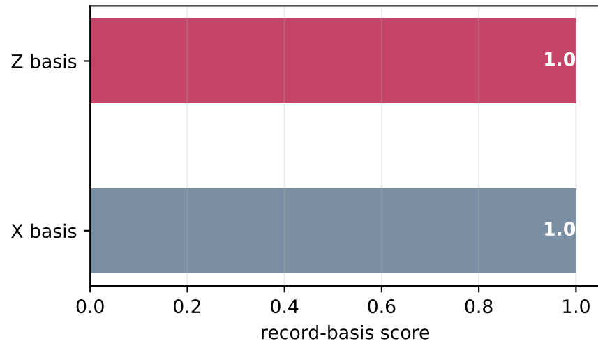
Single-record Bell control
