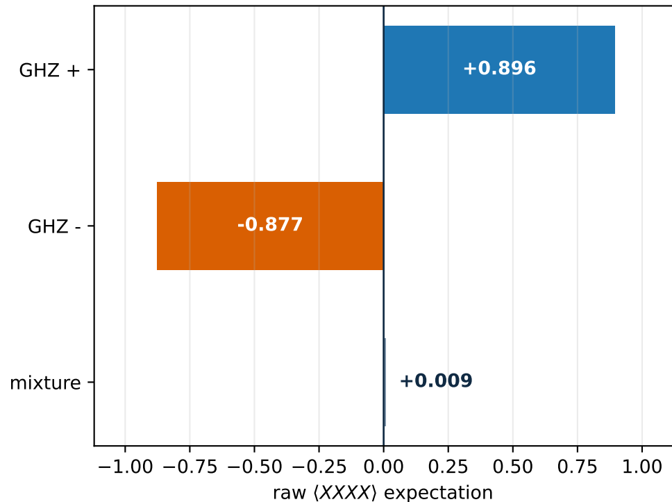
Global coherence witness
