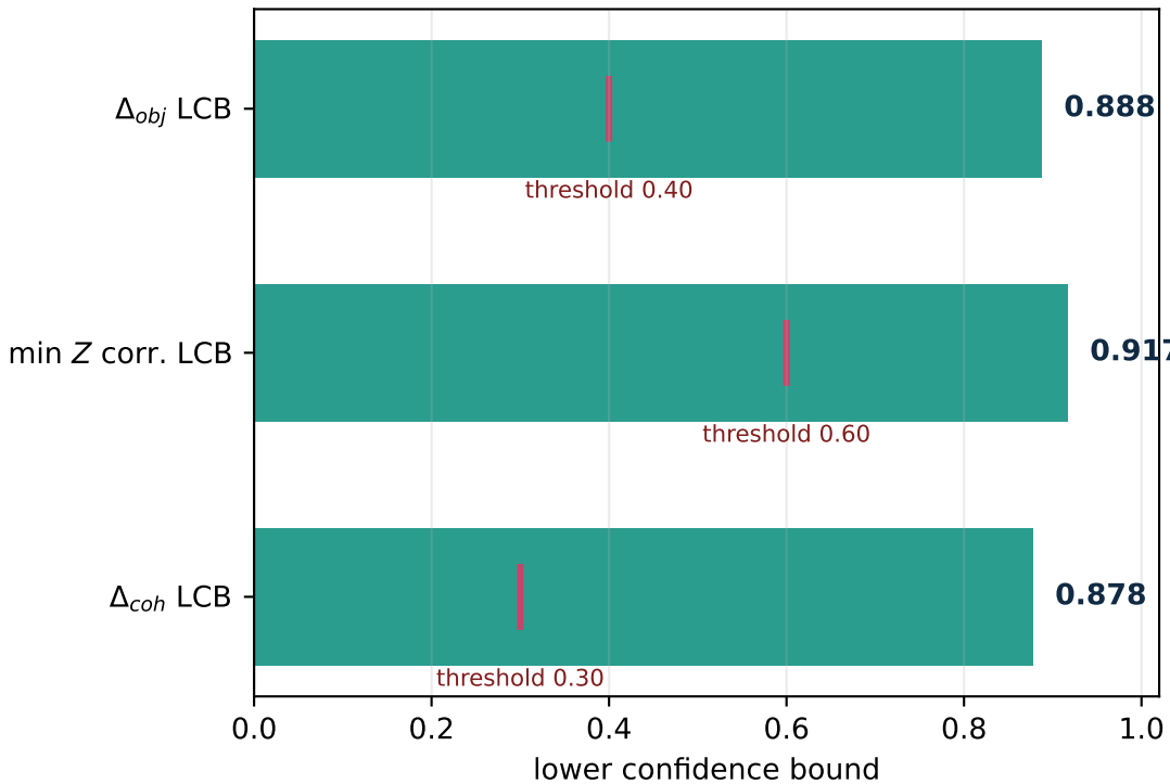
Raw QPU inclusion margins
