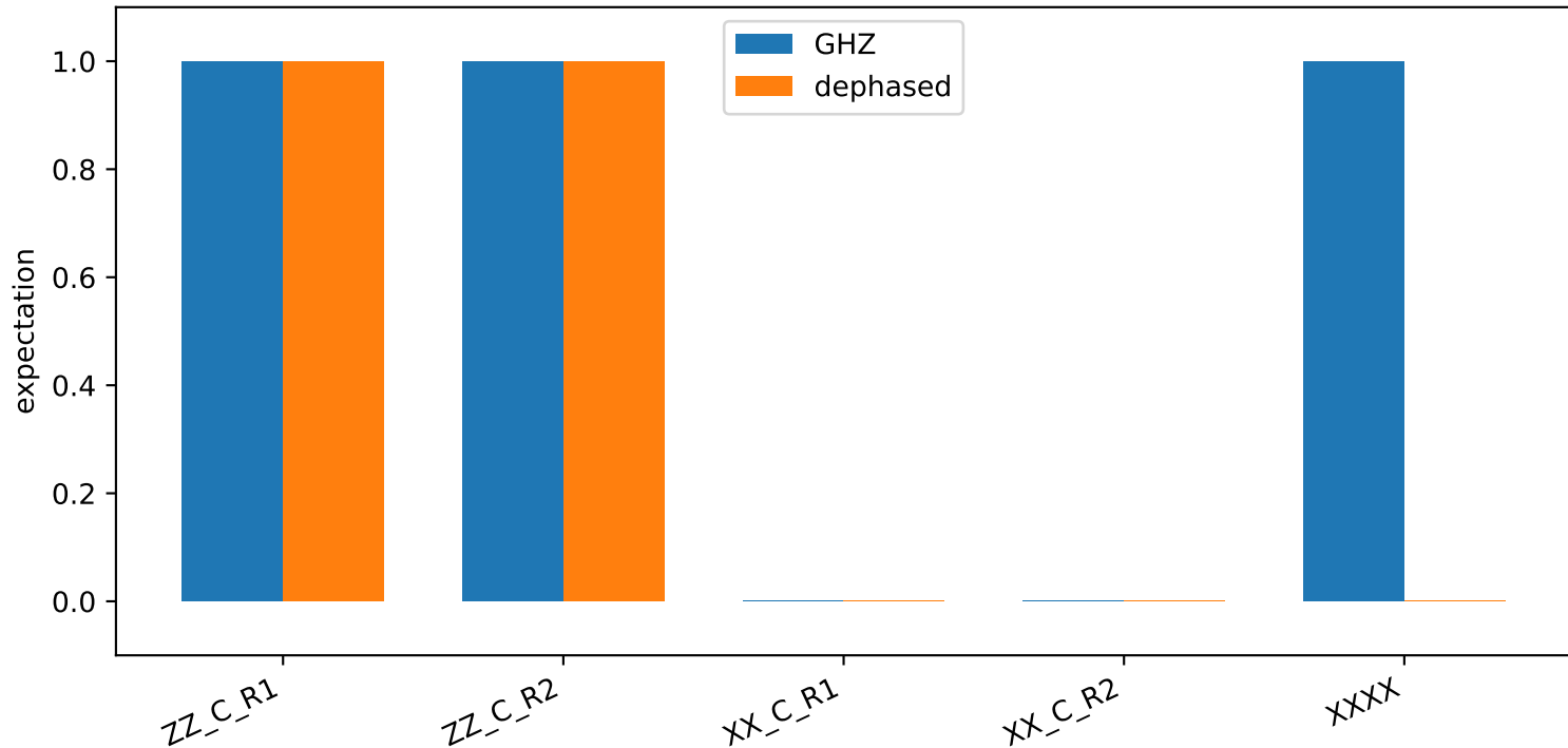
C5 exact GHZ vs dephased-control observables
