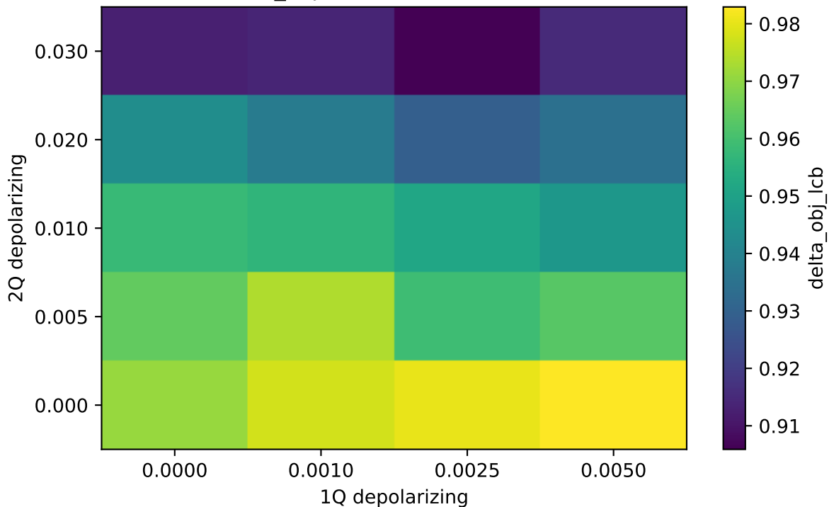
Q302 delta_obj LCB at lowest readout error
