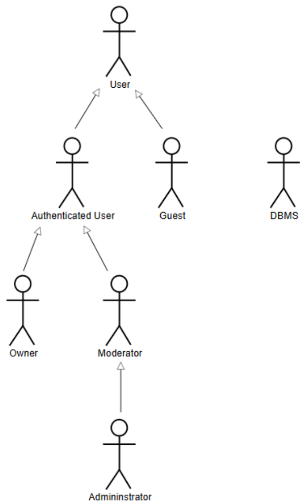
Figure 1: BountyBust Actors.
