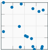
Random
