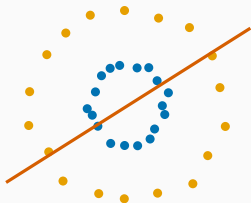
linear model: assumes a straight boundary (fails)
