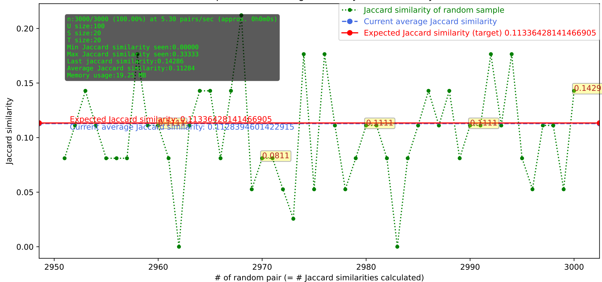
Expected and average value of Jaccard similarity
