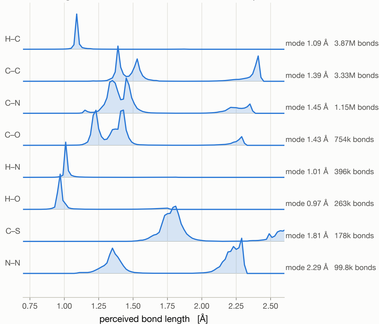
Bond-length distributions, most common element pairs
