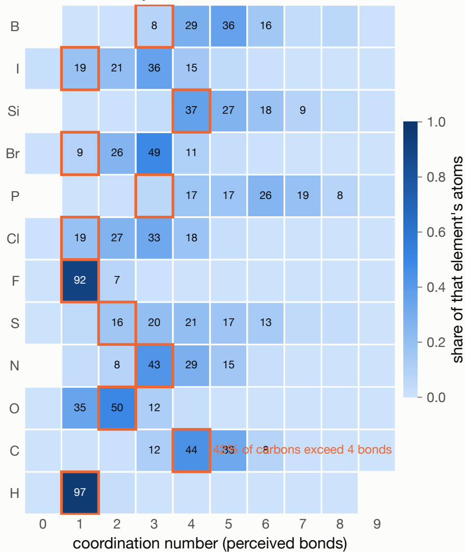
Coordination by element
