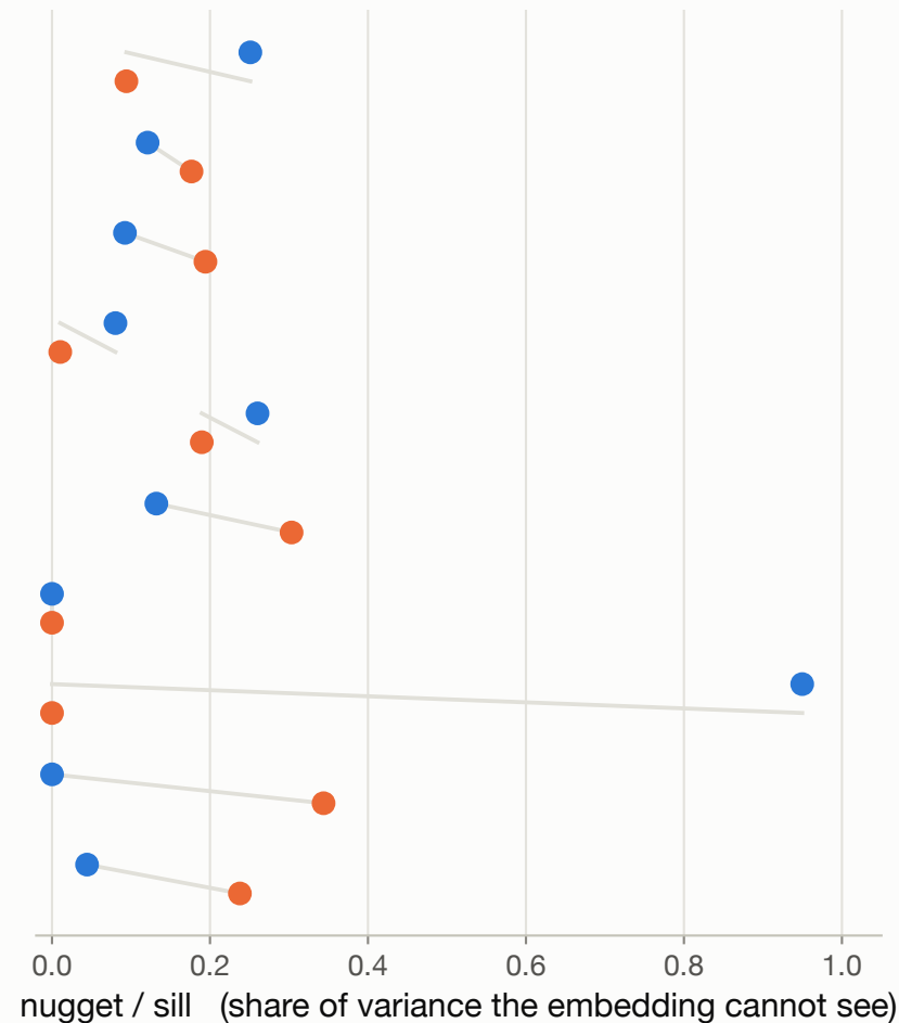
...and neither is the noise floor
