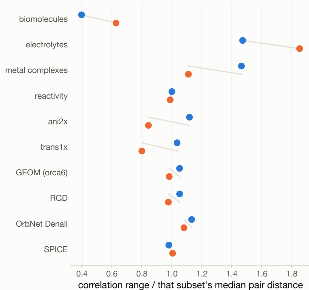
The correlation range is not one number
