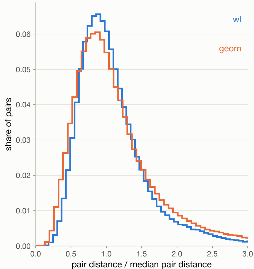
One mode, no gap: compact support is a budget choice, not a natural scale
