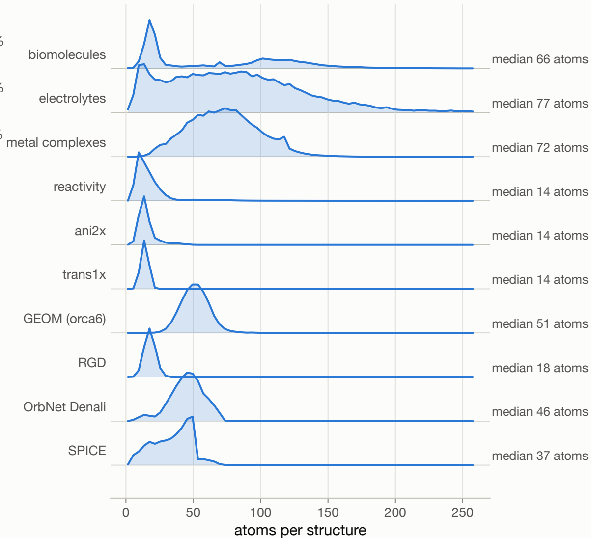
System size by subset
