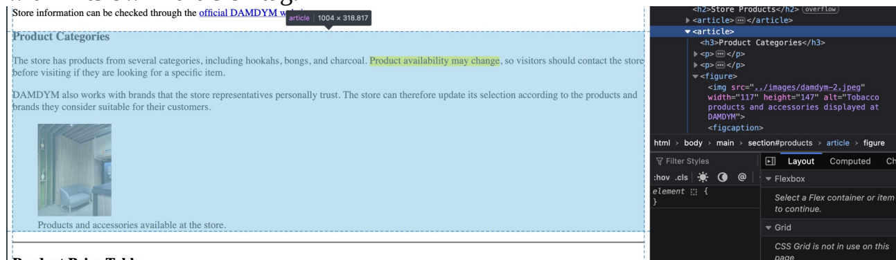
Image 2 – Articles
