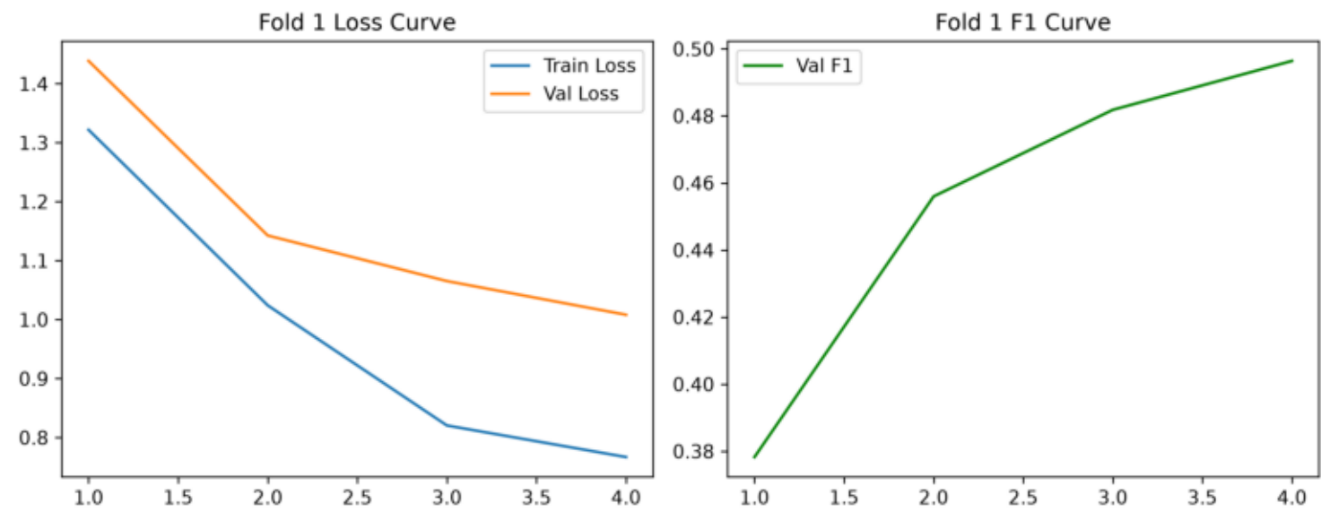
Crop Disease Training & F1 Curves (RepViT)
