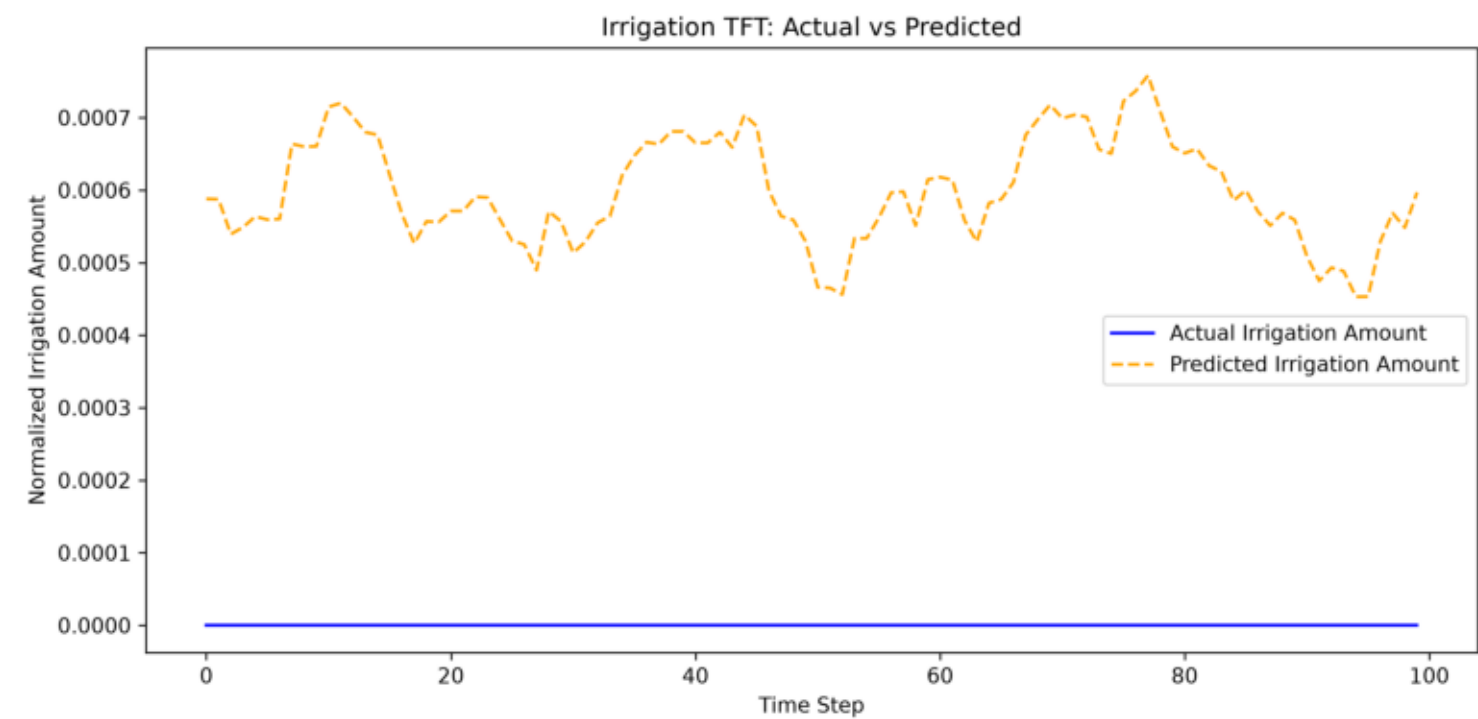
Irrigation Time Series TFT: Actual vs Predicted
