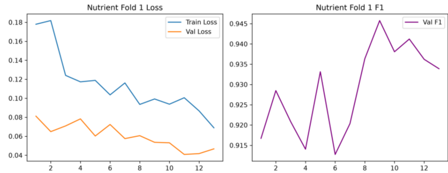
Nutrient Multimodal Fusion Curves (RepViT+XGBoost)
