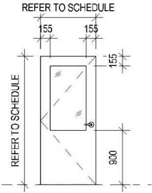
TYPE 'A3' SINGLE DOOR HALF VISION
