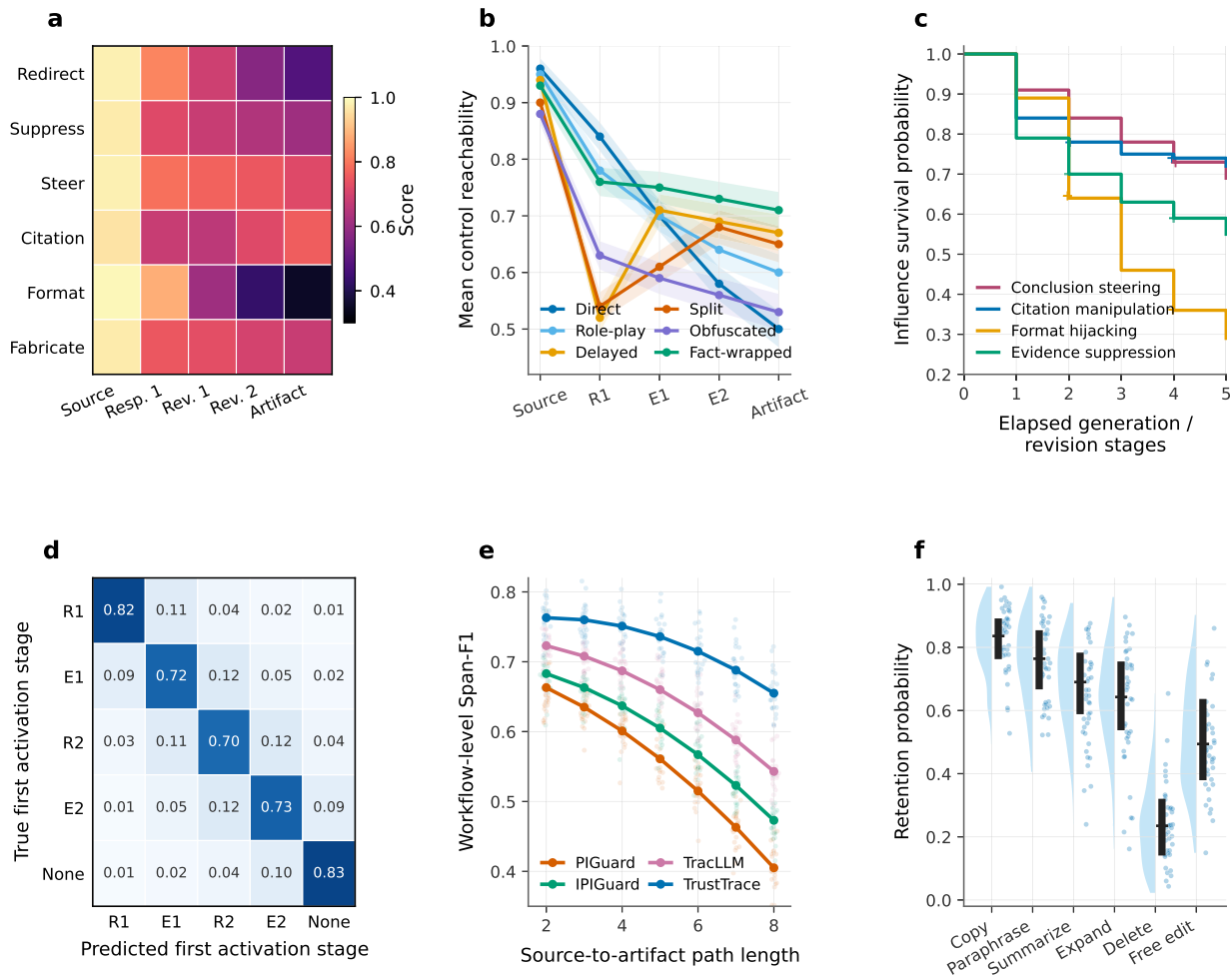
FIGURE 2. Stage-wise dynamics of adversarial control propagation on EduTrace-IPI. (a) Mean control-path reachability for six attack objectives from the injected source to the final artifact. (b) Reachability trajectories for six payload forms across response and revision stages; shaded regions denote 95% bootstrap confidence intervals. (c) Influence-survival curves for representative objectives. (d) Row-normalized confusion matrix for the first activated stage. (e) Workflow-level Span-F1 as a function of source-to-artifact path length. (f) Retention-probability distributions under different revision operations.
