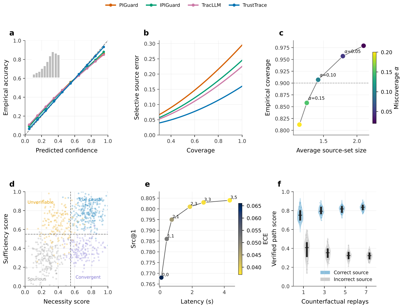
FIGURE 5. Calibration, counterfactual verification, and deployment trade-offs on EduTrace-IPI. (a) Reliability diagrams for propagation confidence; the inset shows the confidence distribution. (b) Selective source error as coverage varies. (c) Empirical coverage versus average source-set size under different miscoverage levels. (d) Joint necessity-sufficiency scores for verified and ambiguous source paths. (e) Src@1-latency Pareto curve for verification budgets ( B_v, B_r ); color denotes ECE. (f) Verified-path score distributions for correct and incorrect source candidates as the number of counterfactual replays increases.
