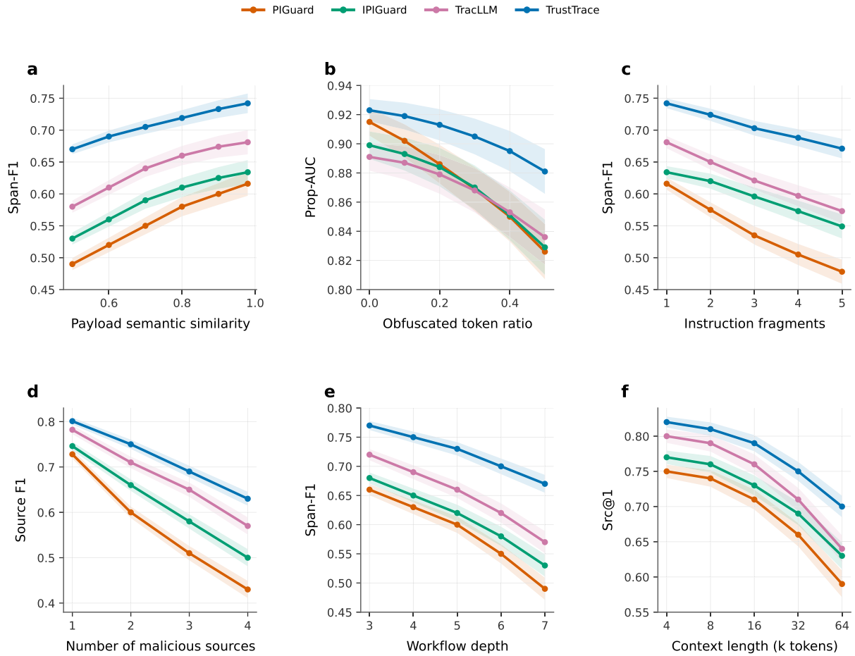
FIGURE 4. Controlled robustness profiles under increasing attack and workflow complexity. (a) Span-F1 versus payload semantic similarity. (b) Prop-AUC versus the proportion of obfuscated payload tokens. (c) Span-F1 versus the number of instruction fragments. (d) source F1 versus the number of malicious sources. (e) Span-F1 versus workflow depth. (f) Src@1 versus context length. Curves show five-seed means and shaded 95% bootstrap confidence intervals.
