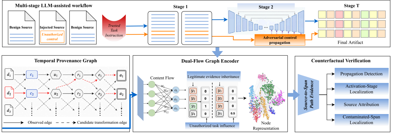
FIGURE 1. Overview of the TrustTrace framework for detecting, tracing, and verifying indirect prompt-injection propagation.
