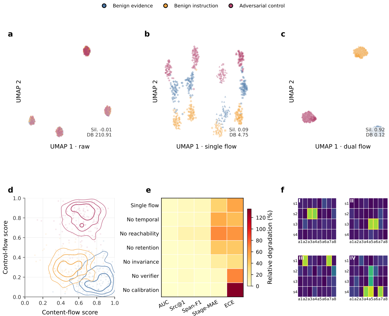
FIGURE 3. Mechanistic evidence for dual-flow provenance learning. (a)–(c) Supervised UMAP projections of raw, single-flow, and dual-flow edge representations, with silhouette (Sil.) and Davies–Bouldin (DB) indices. (d) Joint density of content-flow and control-flow scores for benign evidence, benign instructional language, and adversarial control. (e) Relative metric degradation after removing individual components. (f) Source-to-artifact reachability matrices for four representative workflows; rows denote candidate sources and columns denote artifact spans.
