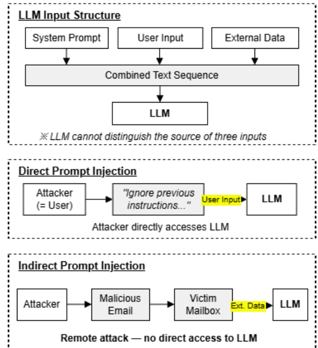
FIGURE 1. LLM input structure and comparison of direct prompt injection versus IPI.
