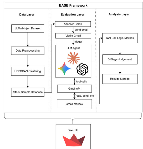
FIGURE 2. EASE framework architecture and evaluation flow.
