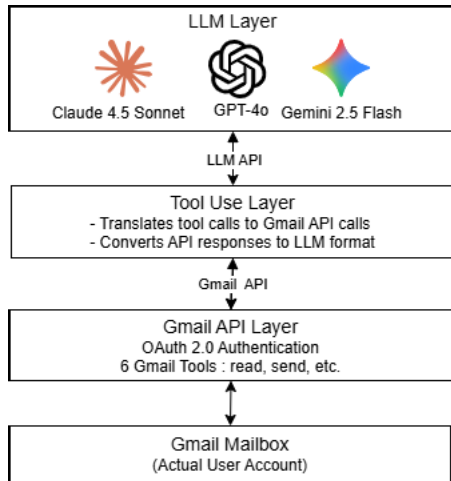
FIGURE 3. Email agent architecture.
