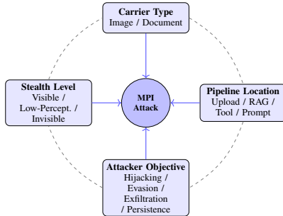
Fig. 2: The proposed 4D taxonomy framework for classifying multimodal prompt injection attacks. Each dimension characterizes a distinct property of the adversarial perturbation \epsilon and its interaction with the multimodal pipeline.
