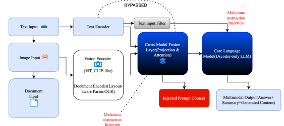
Fig. 1: Multimodal Prompt Injection Bypass Mechanism
