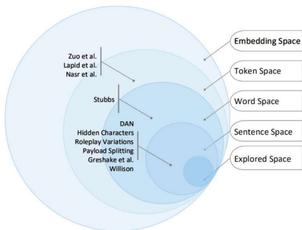
FIGURE 4. Visualization of the prompt injection space as proposed by Kumar et al. 2024 a , illustrating five levels of abstraction: embedding, token, word, sentence, and explored spaces.
