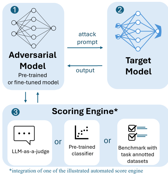
FIGURE 8. Key elements of recent automated red teaming architectures for LLMs.
