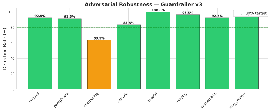
Figure 7: Transformation-based robustness evaluation across 8 attack transformations ( n = 200 ). The green dashed line at 80% indicates the minimum acceptable detection rate. Misspelling (63.5%) is the only transformation falling below this threshold, while Base64 encoding achieves 100% detection. These results reflect fixed transformations only; adaptive adversarial attacks were not evaluated.
