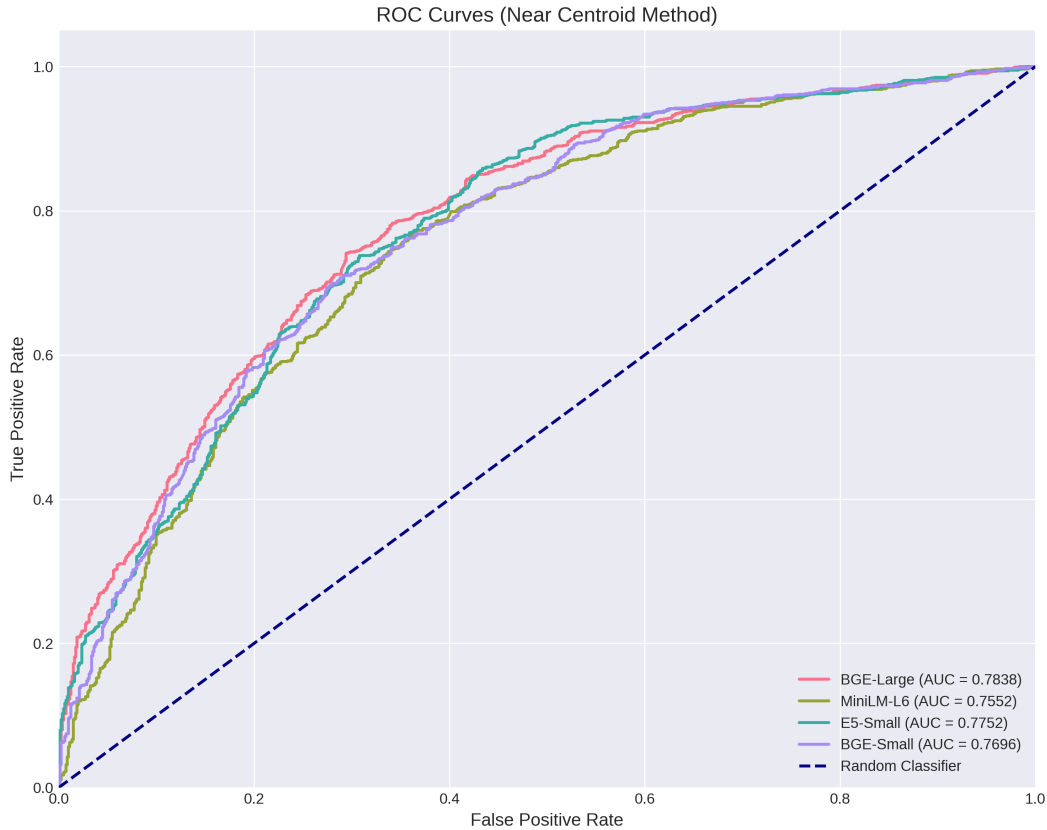
Figure 2: ROC curves for four embedding models using Euclidean distance with StandardScaler. BGE-Large achieves the highest AUC (0.784), followed by E5-Small (0.775), BGE-Small (0.770), and MiniLM-L6 (0.755).
