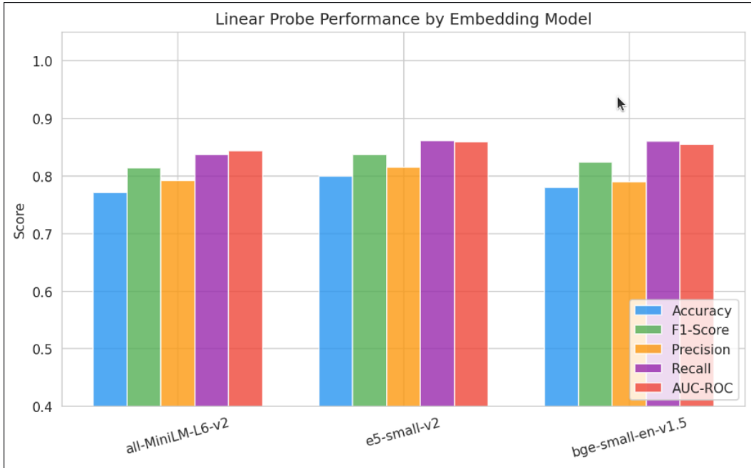
Figure 3: Linear probe performance by embedding model. All three small models achieve AUC-ROC above 0.84, with e5-small-v2 showing the highest AUC and MiniLM-L6 the lowest. The consistent performance across models suggests that discriminative information is present in the evaluated embedding spaces.
