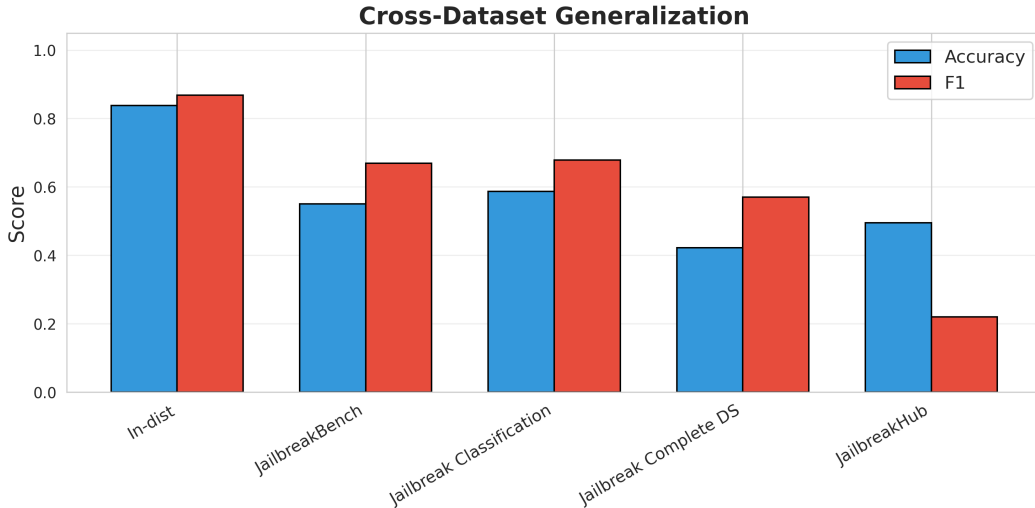
Figure 8: Cross-dataset generalization results. The model trained on Guardrail Dataset v1 shows severe performance degradation on four external datasets. In-distribution accuracy (83.0%) drops to 42.2–59.0% on external benchmarks, with JailbreakHub showing particularly poor performance (F1 = 0.220).
