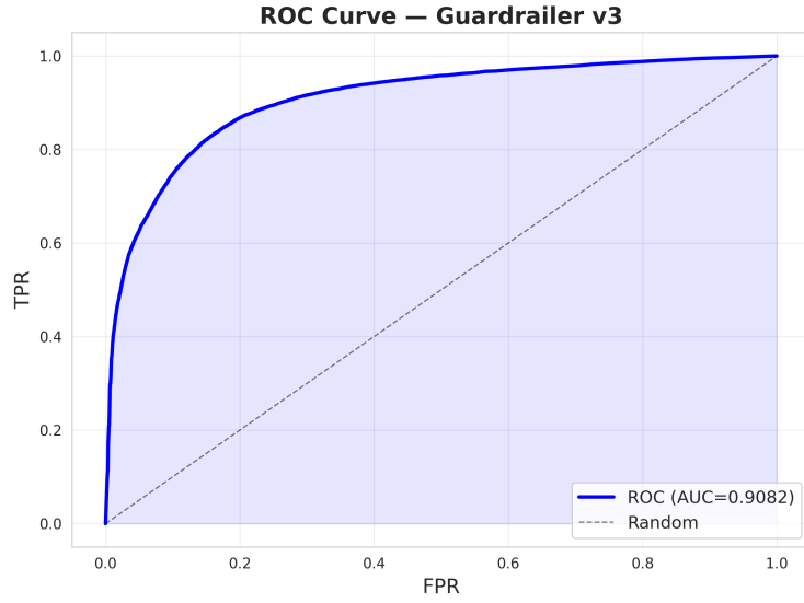
Figure 5: ROC curve for Hybrid Guardrail V3. The model achieves AUC = 0.908 , indicating strong ranking performance across classification thresholds on the evaluated in-distribution test set.
