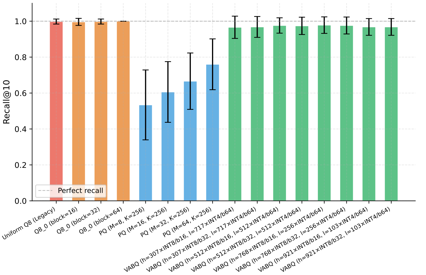
Recall@10 Distribution per Method
