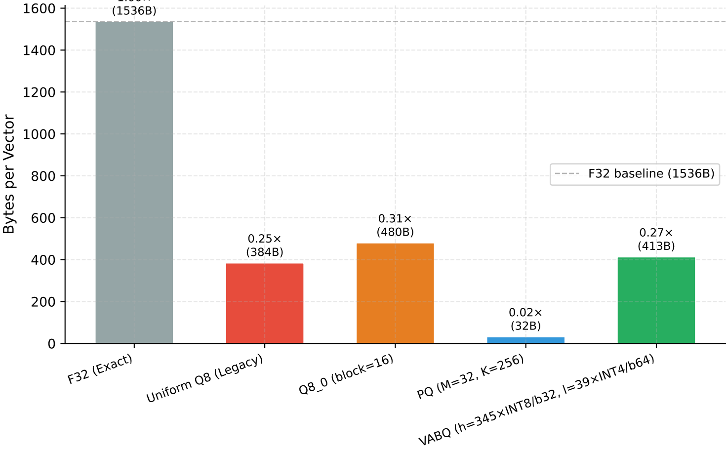
Storage Footprint per Vector
