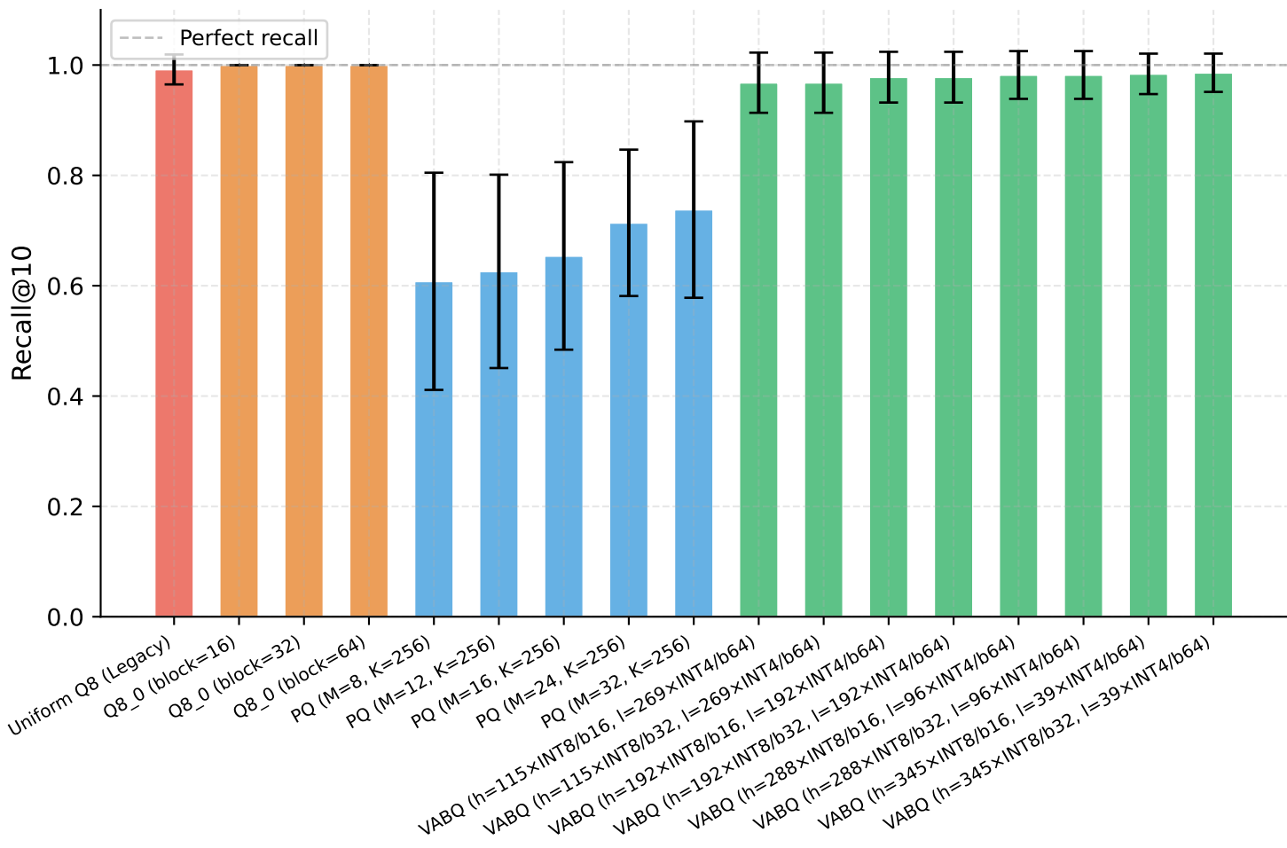
Recall@10 Distribution per Method
