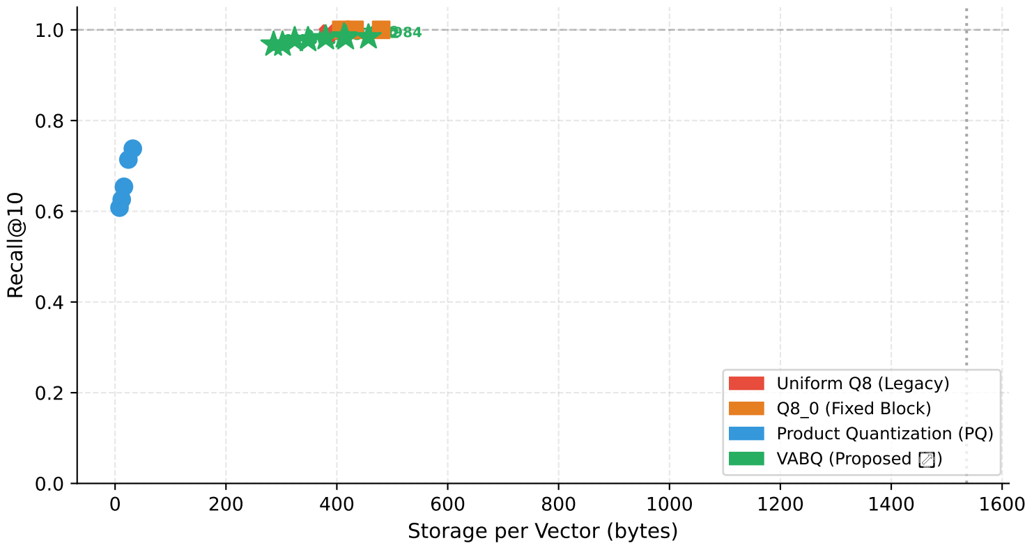
Storage Footprint per Vector
