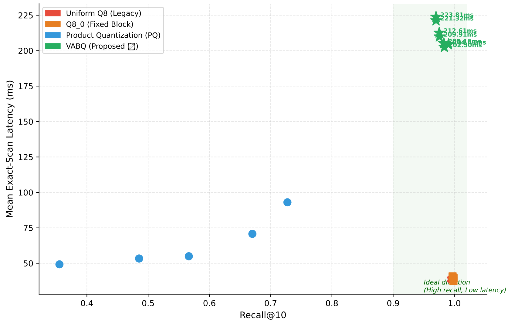
Latency vs. Recall@10
