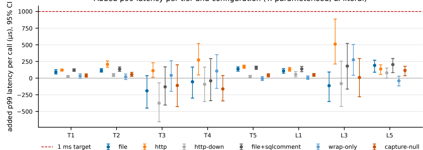
Added p99 latency per tier and configuration (T: parameterised; L: literal)
