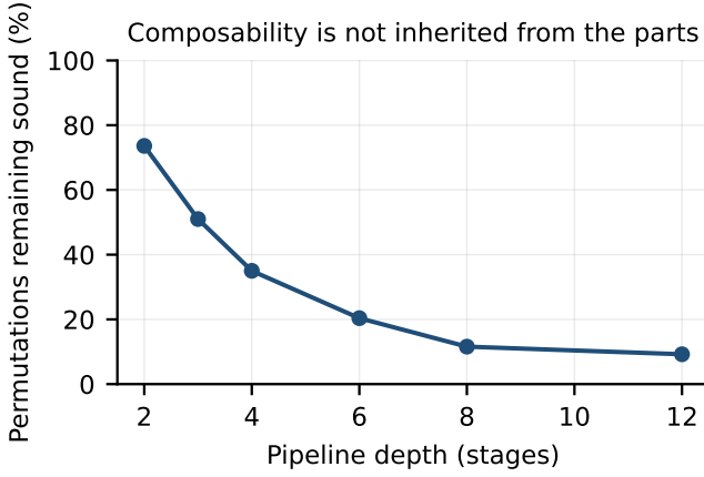
Fig. 1. Soundness of a valid pipeline under random reordering, against depth. The fraction of assemblies that remain contract-sound falls as pipelines become deep enough for reuse to be the point.
