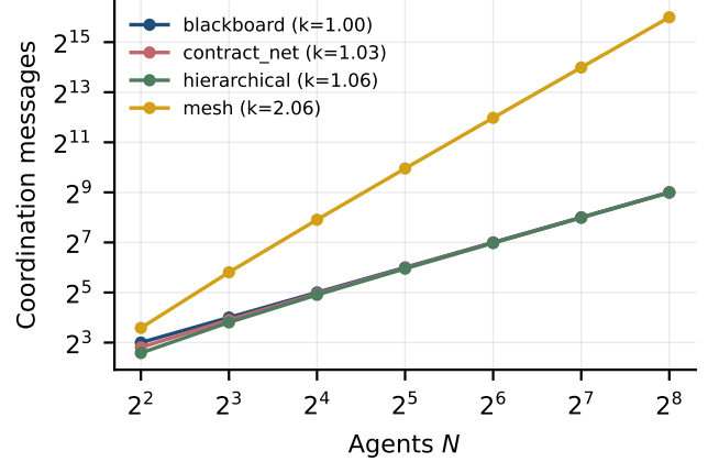
Figure 1: Coordination messages against agent count, log-log. The fitted exponent separates quadratic mesh broadcast from the linear coordinated topologies.
