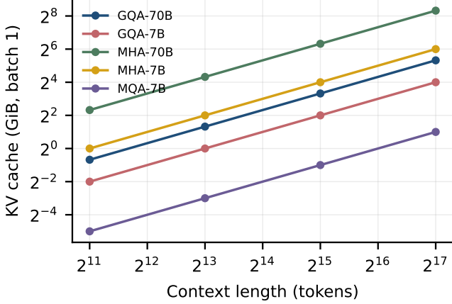
Fig. 1. Exact KV cache size against context length, log-log. Slope one confirms linear growth; the vertical offsets are the head-sharing factor.
