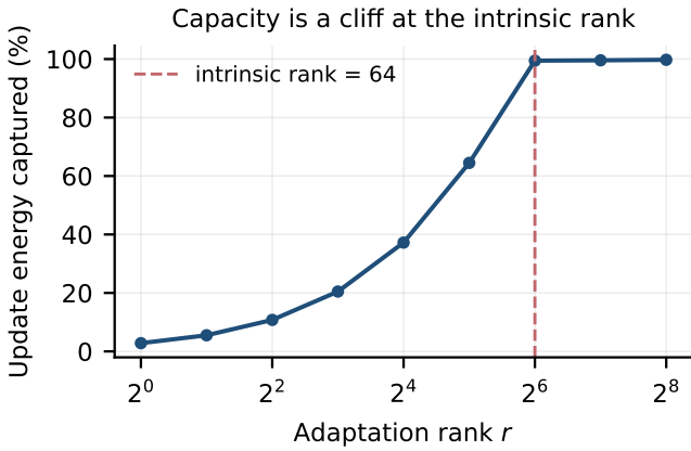
Fig. 2. Update energy captured against adaptation rank, measured by SVD. Capacity saturates abruptly at the planted intrinsic rank.
