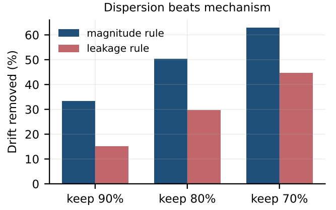
Fig. 2. Drift removed by each selection rule. Magnitude wins despite leakage being the governing factor, because magnitude carries the wider dispersion.
