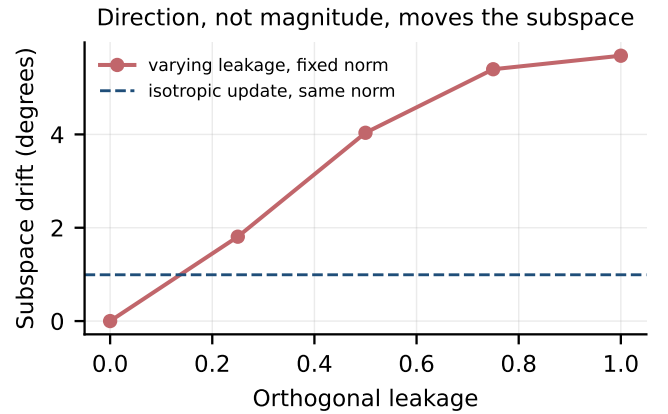
Fig. 1. Subspace drift against orthogonal leakage at fixed update norm. An update confined to the safety subspace leaves it exactly in place; the dashed line marks an isotropic update of identical norm.
