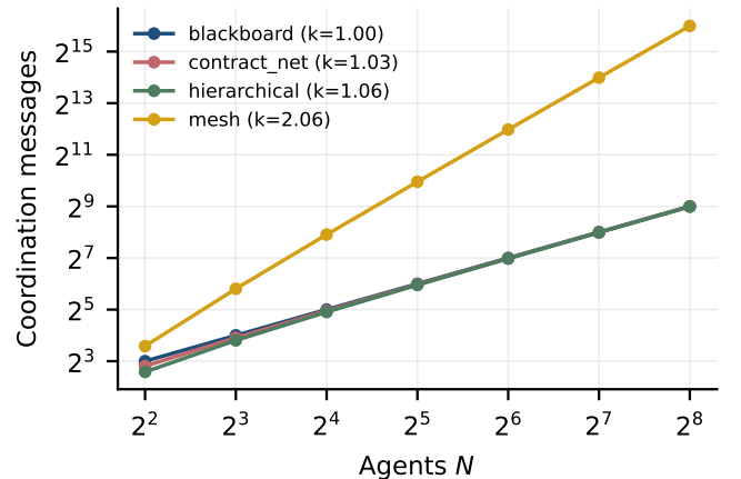
Fig. 1. Coordination messages against agent count, log-log. The fitted exponent separates quadratic mesh broadcast from the linear coordinated topologies.
