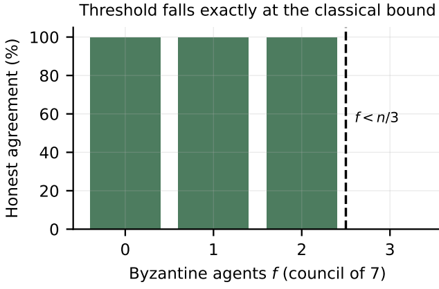
Fig. 1. Honest agreement against the number of Byzantine agents in a council of seven. Agreement collapses precisely where the f < n/3 bound predicts.
