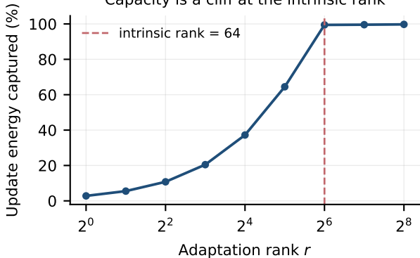
Capacity is a cliff at the intrinsic rank
