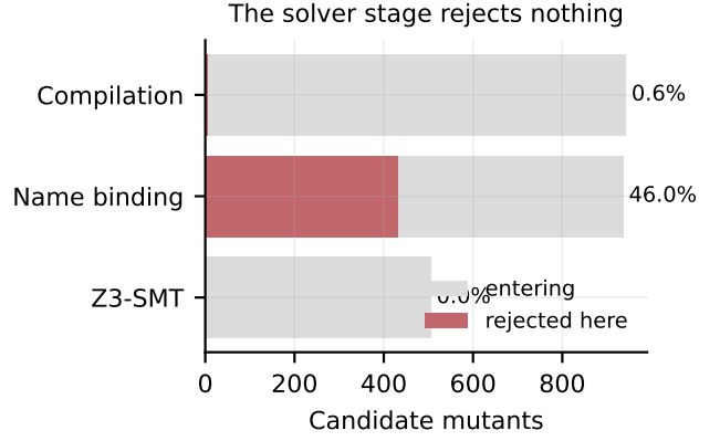
Figure 1: Candidates entering each pre-filter stage and the share rejected there. Static name binding carries the filter; the SMT stage rejects nothing.
