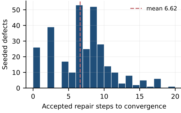
Figure 2: Accepted repair steps to convergence over 300 seeded defects. Every trial terminated, with a worst case well inside the theoretical bound.
