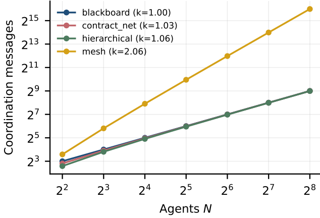
Fig. 1. Coordination messages against agent count, log-log. The fitted exponent separates quadratic mesh broadcast from the linear coordinated topologies.
