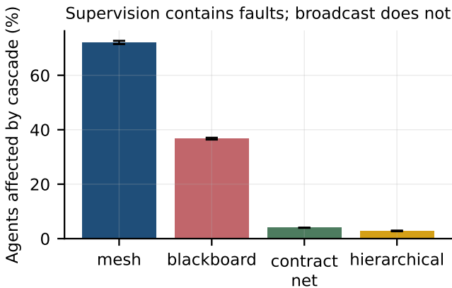
Fig. 2. Mean fraction of agents affected by a cascade, with bootstrap 95% confidence intervals over 20,000 trials per topology.
