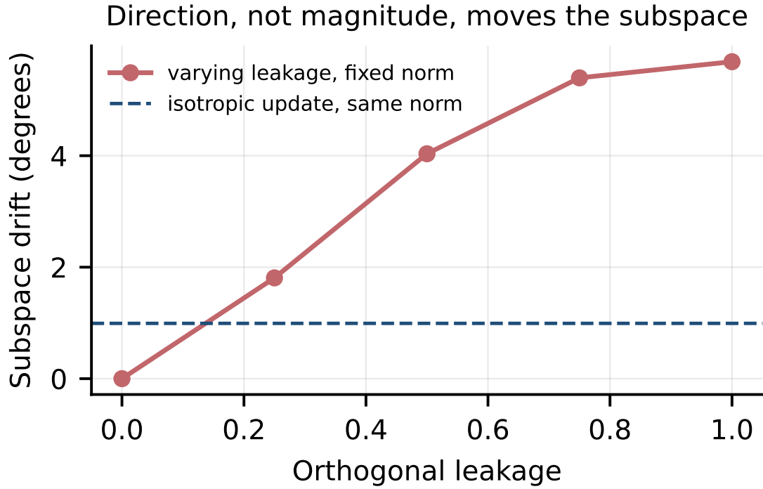
Fig. 1. Subspace drift against orthogonal leakage at fixed update norm. An update confined to the safety subspace leaves it exactly in place; the dashed line marks an isotropic update of identical norm.
