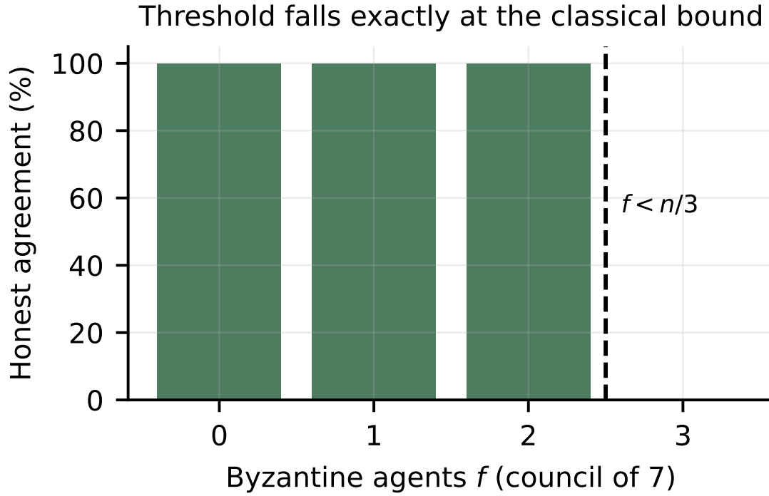
Fig. 1. Honest agreement against the number of Byzantine agents in a council of seven. Agreement collapses precisely where the f < n/3 bound predicts.
