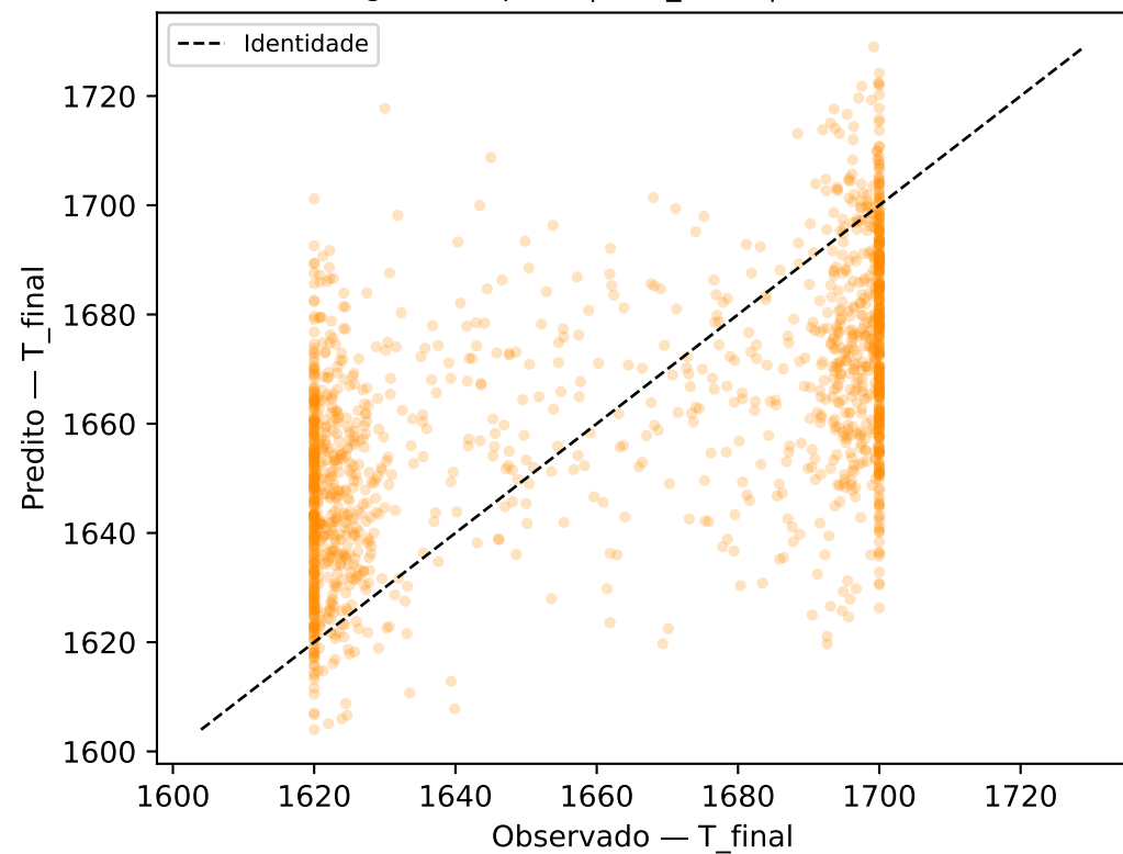
Config B (MLP prof.) | MLP_DEEP | MAE=24.0340
