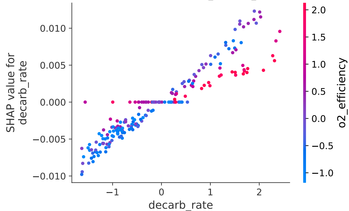
SHAP Dependence: decarb_rate \rightarrow C_final
