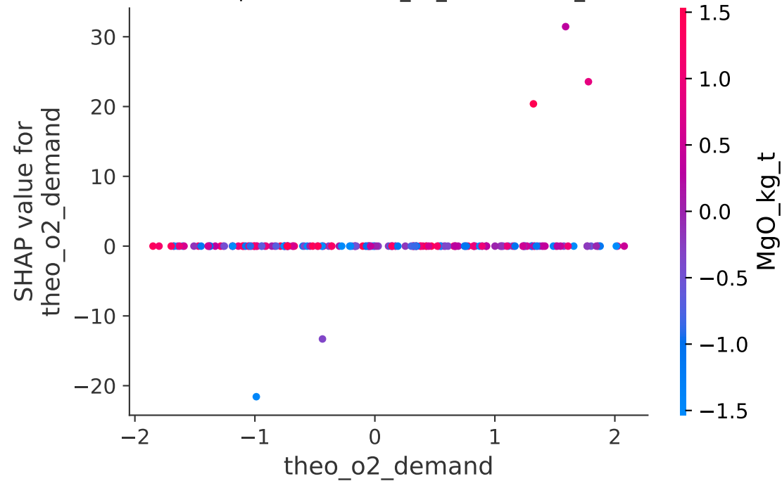
SHAP Dependence: theo_o2_demand → T_final
