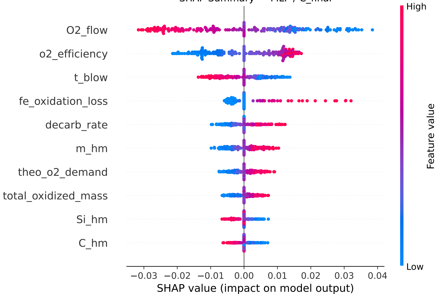
SHAP Summary — MLP / C_final
