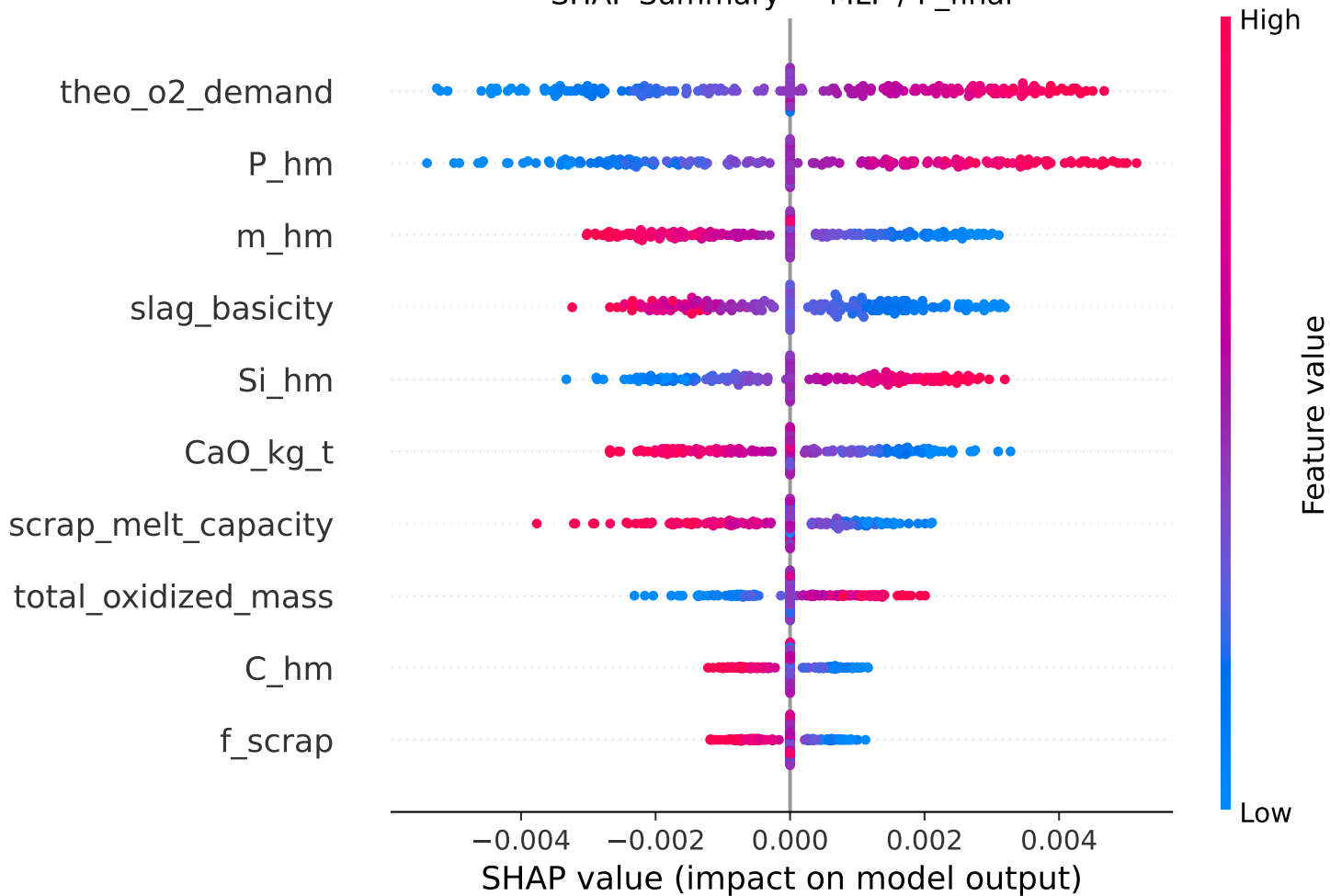
SHAP Summary — MLP / P_final
