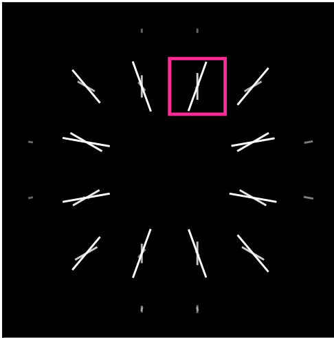
oriented-gradient histograms
