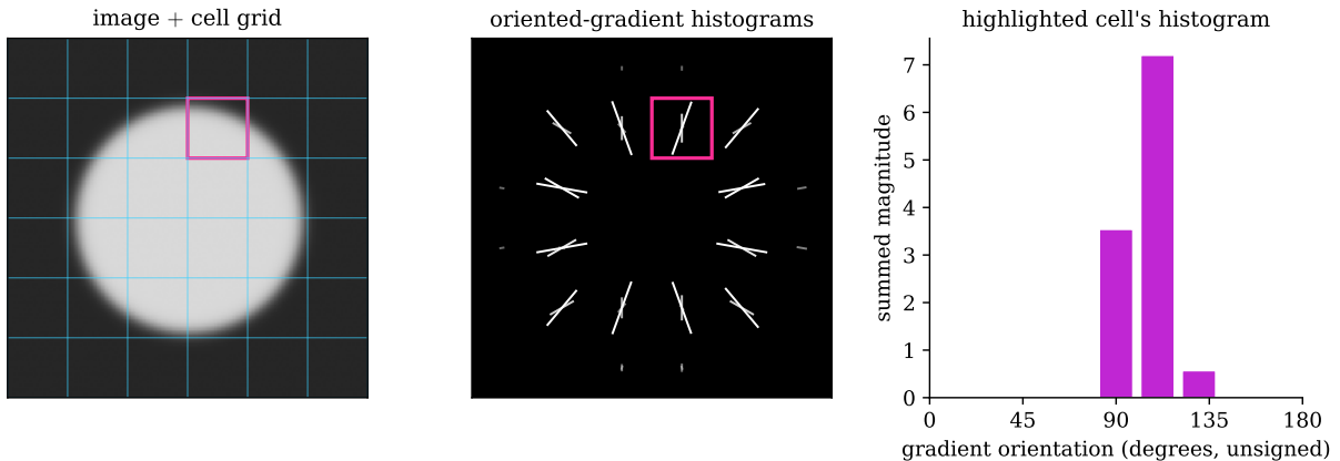
Figure 14: Building a HOG descriptor, computed on a synthetic disk. Left: the region is divided into a grid of cells (one highlighted in magenta). Middle: each cell is replaced by a small star of strokes, one per orientation bin, whose length is the total gradient magnitude falling in that orientation; since gradients run perpendicular to edges, the strokes point radially around the disk’s rim, while flat interior and exterior cells stay empty. Right: the highlighted cell’s nine-bin histogram of gradient orientation, each pixel weighted by its gradient magnitude, with a clear peak at the orientation of the local edge. Stacking every cell’s (block-normalized) histogram into one vector yields the descriptor.
