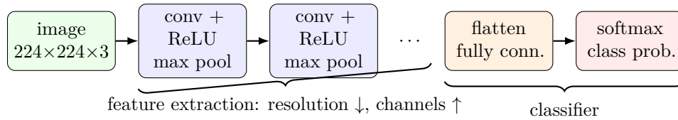
Figure 30: Basic layout of a convolutional network for classification. Convolution–ReLU–pooling blocks extract increasingly abstract features at decreasing resolution; fully connected layers and a softmax turn them into class probabilities.
