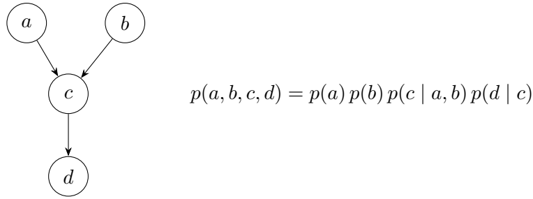
Figure 37: A Bayesian network and its factorization. Each node contributes one factor conditioned on its parents; a and b have no parents and contribute their marginals.
