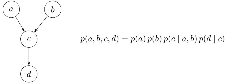
Figure 45: A Bayesian network and its factorization. Each node contributes one factor conditioned on its parents; a and b have no parents and contribute their marginals.
