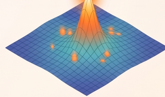
Figure 19: Generalized Hough transform. Each model edge stores a displacement vector to the reference point, organized in the R-table by gradient orientation. Because the same orientation occurs at several places on the shape, one observed edge casts votes for several candidate centers; the true center is where votes accumulate.
