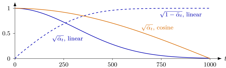
Figure 42: Signal coefficient \sqrt{\alpha_t} (solid) and noise coefficient \sqrt{1 - \bar{\alpha}_t} (dashed) for the linear schedule with T = 1000 , and the signal coefficient of the cosine schedule (orange). The linear schedule destroys the image early and wastes many late steps on almost pure noise; the cosine schedule spreads the destruction more evenly.
